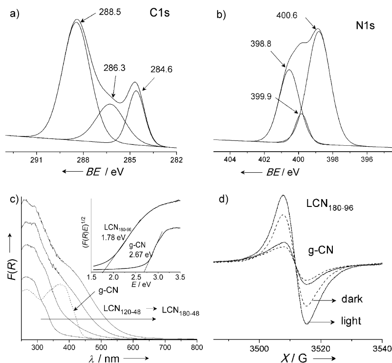
Figure 2. a,b) Core-level XPS spectra of C1s (a) and N1s (b) of LCN 180-96 (BE=binding energy); c) UV/Vis diffuse reflectance spectra of LCN 180-96 and g-CN. The inset shows the bandgap determination of g-CN and LCN 180-96 from the Tauc plots. d) Solid-state ESR spectra of LCN 180-96 and g-CN with visible light or in the dark ( X =magnetic field strength).
